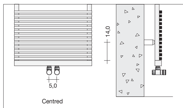
Technical diagram for BA15K i5 connection
